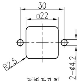
面板开孔图 Panel cut out
